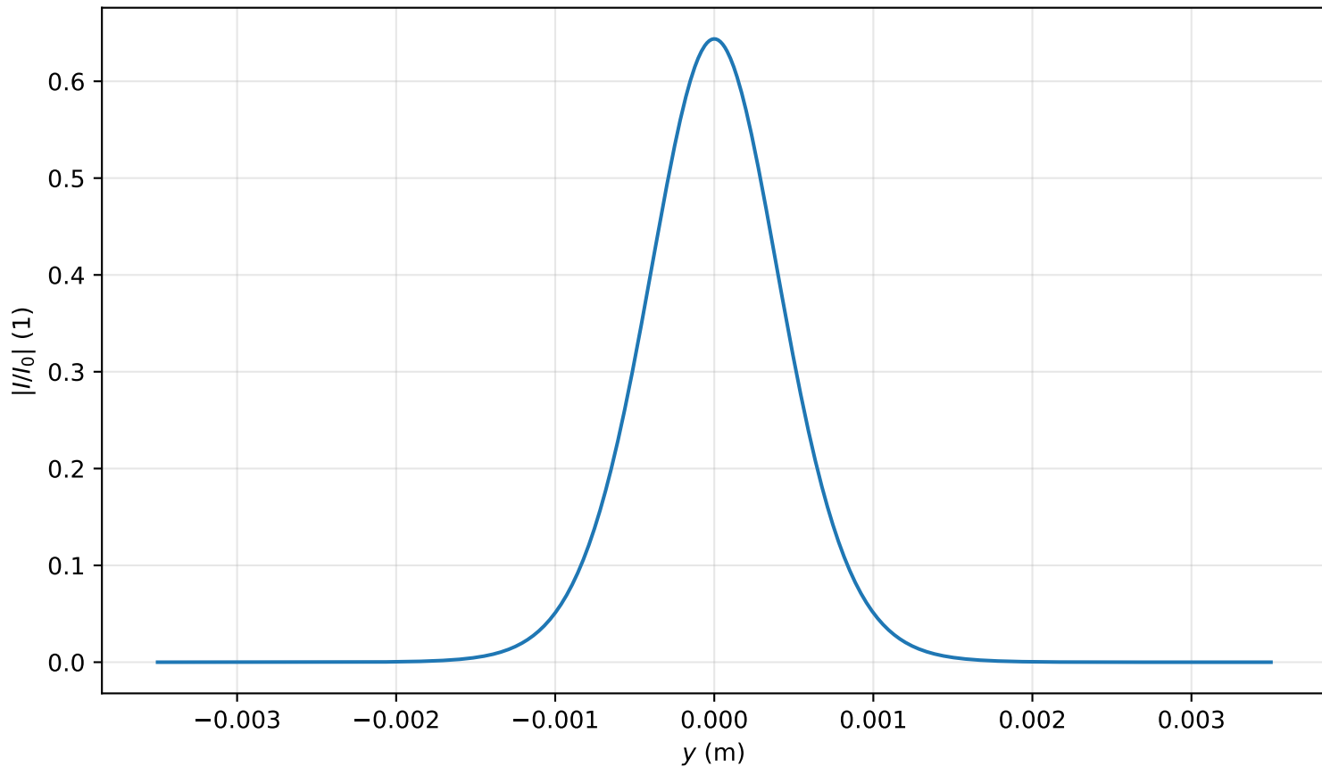
Intensity profile I(x=0, y, z=2.309)/I_0 , P_{in}=0.4P_{cr} , artificial time
